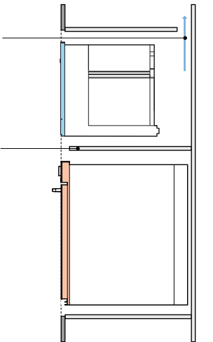
STACK EXPLODED PROFILE VIEW
