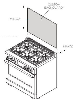
CUSTOM FABRICATED* BACKGUARD *Fabricated from non combustibile materials only
