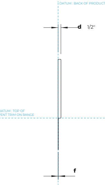
PROFILE VIEW
