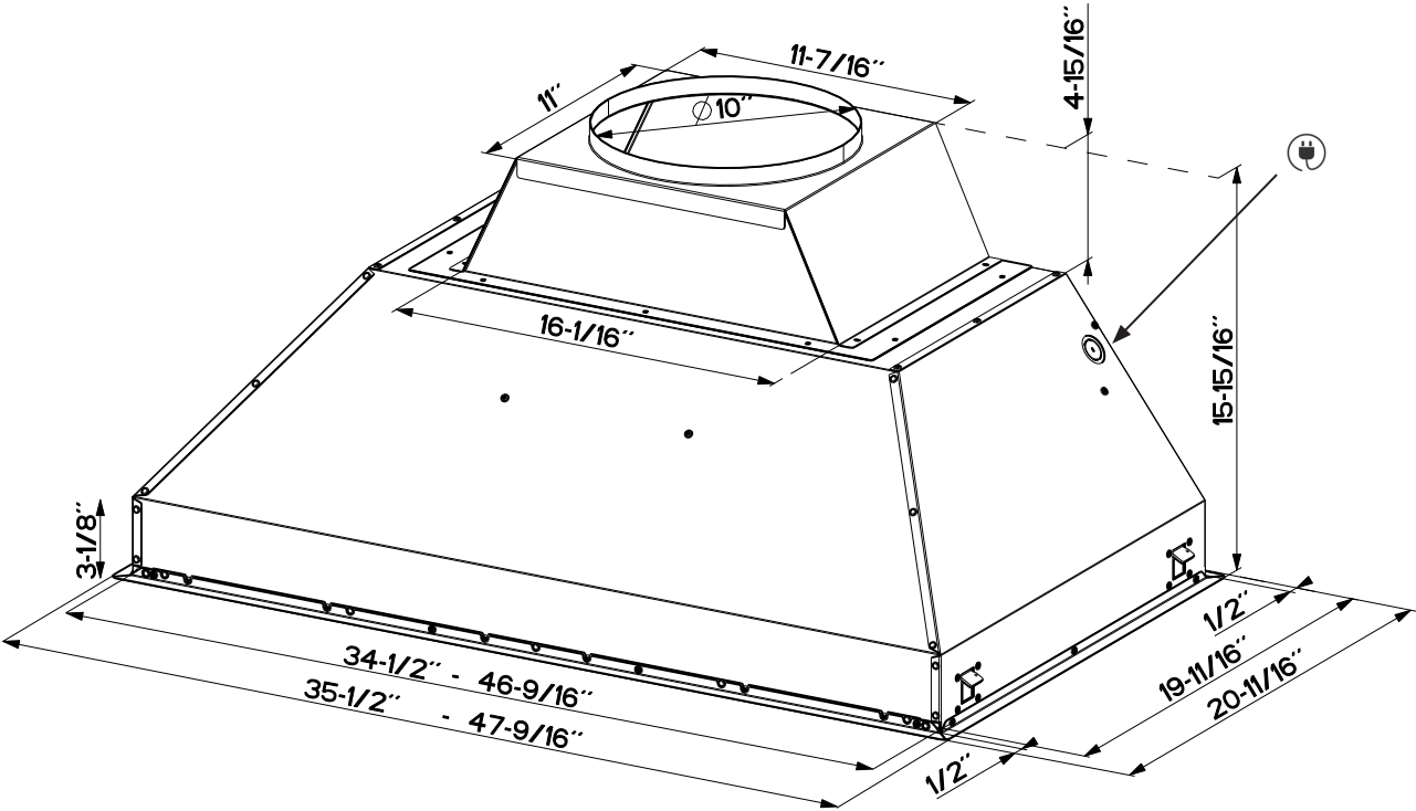
FRONT VIEW
