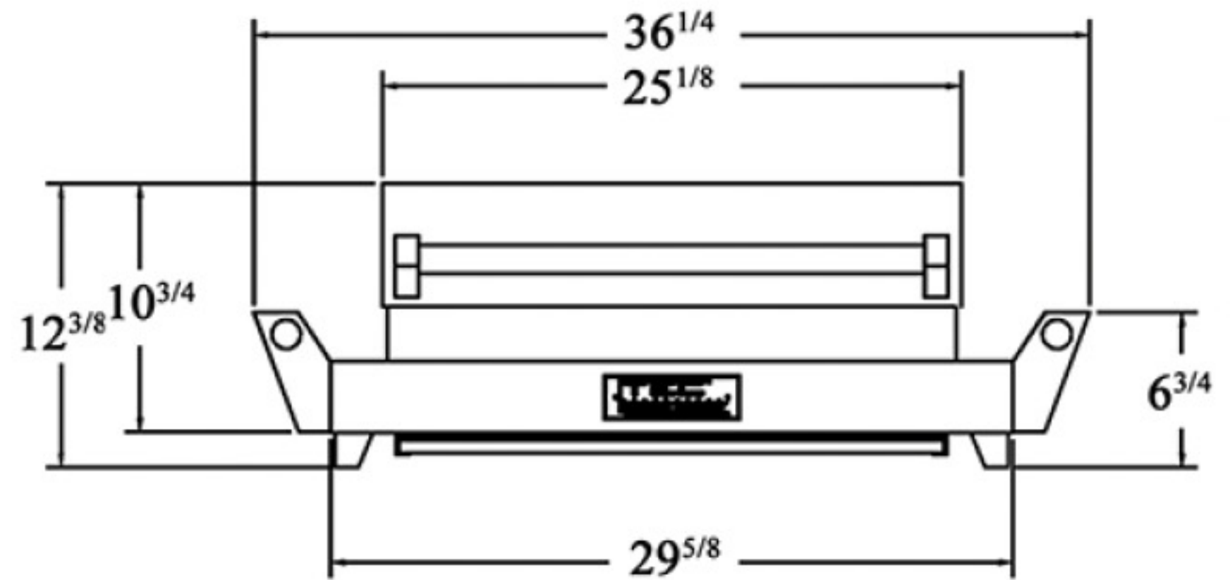
FRONT VIEW
