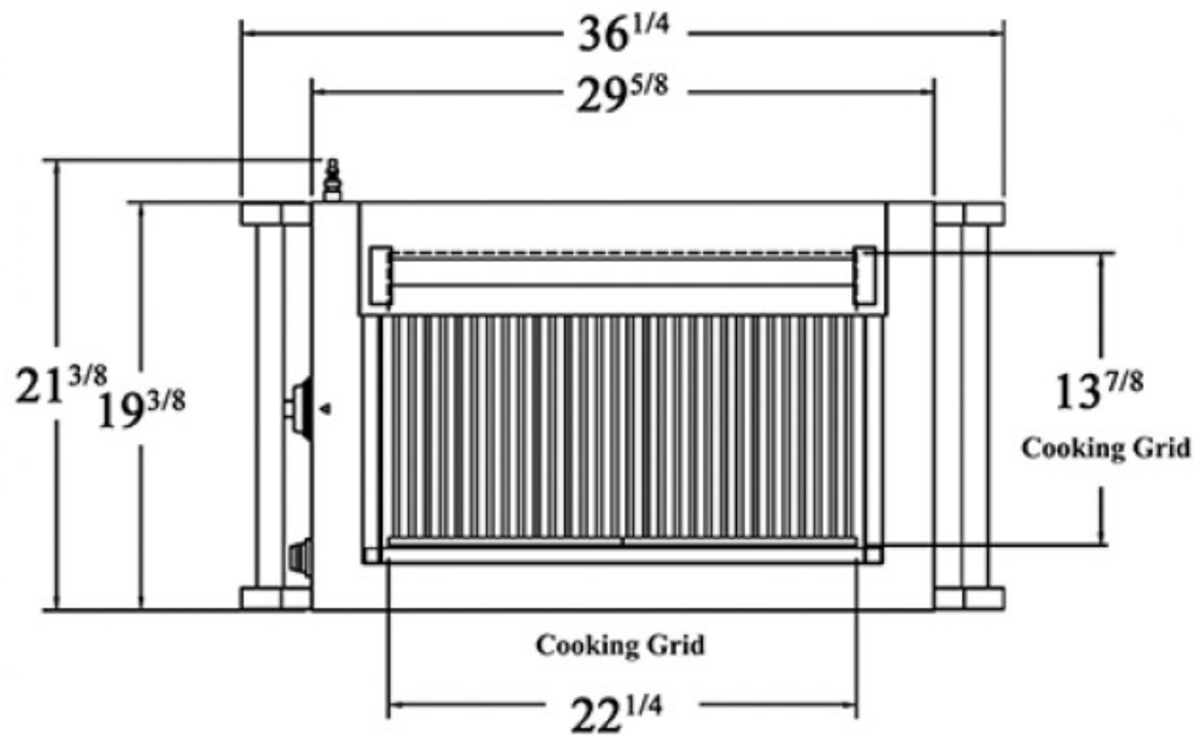
TOP VIEW (SHOWN WITH HOOD OPEN)
