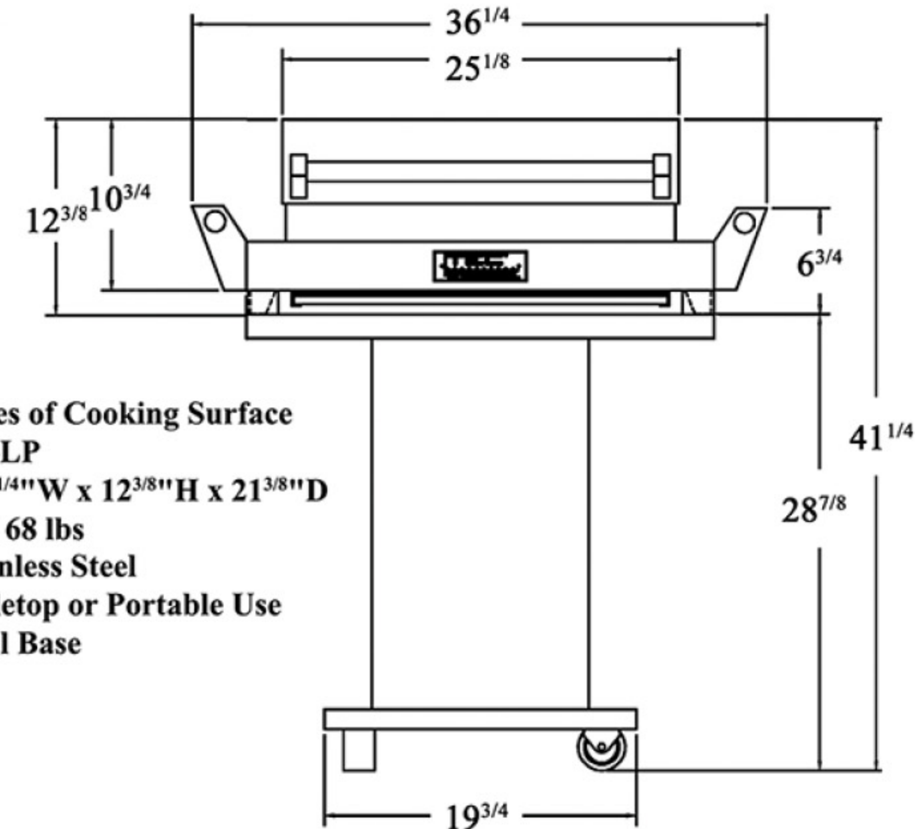
FRONT VIEW
