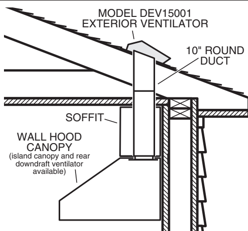
TYPICAL ROOF MOUNTED INSTALLATION
