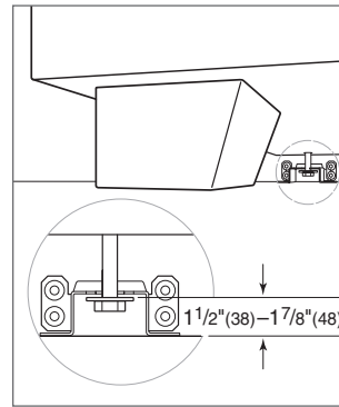
Anti-tip bolt engaged
