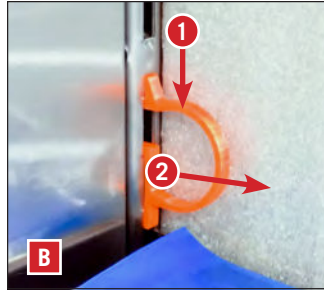
FIG. 3. Remove the shelf shipping clip (A) from the shelf standard (B).
