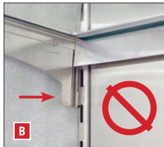
FIG. 5. Underside view. Left side shown. A: CORRECT; Bottom tab is fully seated in the shelf standard. B: INCORRECT; Bottom tab is not seated in the shelf standard.
