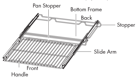
Extendable Rack (Optional)
