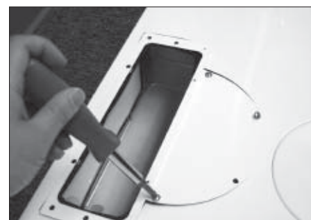
4. Mount rectangular transition piece to top opening as shown.
