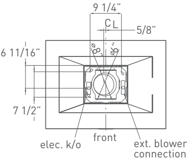
Top (blower housing and ceiling bracket)
