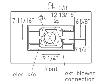
Top (blower housing and ceiling bracket)
