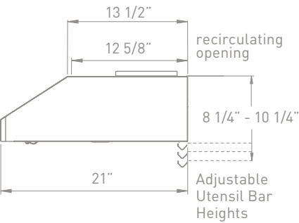
SIDE
