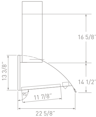
SIDE
