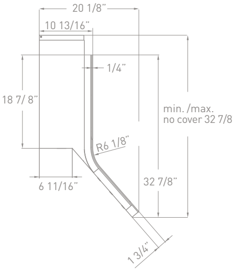
SIDE
