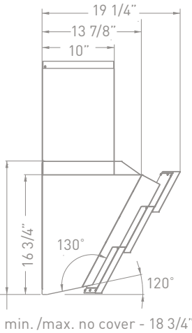
SIDE
