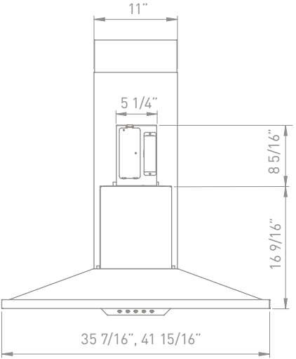
FRONT
