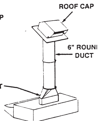
FIG. F. Straight up through the roof using 6" round duct (for single-story installations).
