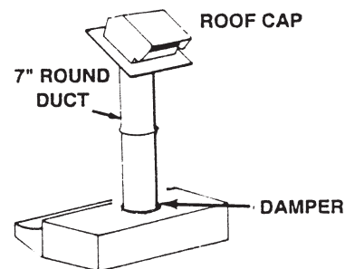
FIG. C. Straight up through the roof using 7" round duct (for single story installations - UXT2030AA and UXT2036AA only)
