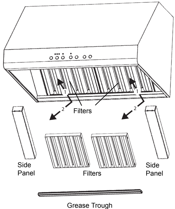
Figure 3: The hood and parts
