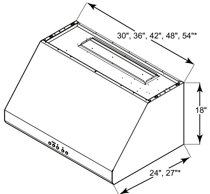
Figure 2: Overall Dimensions
