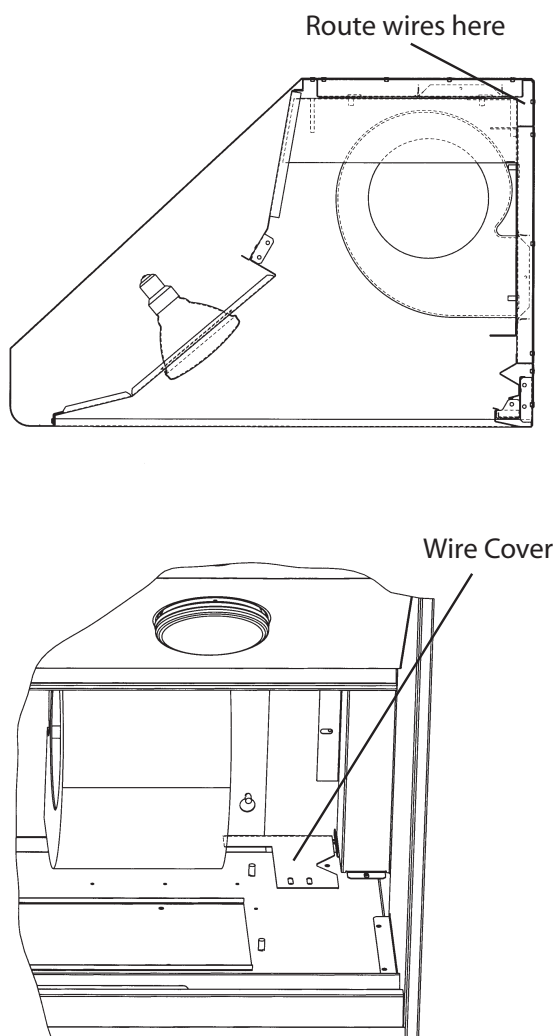
Figure 18: Horizontal Discharge
