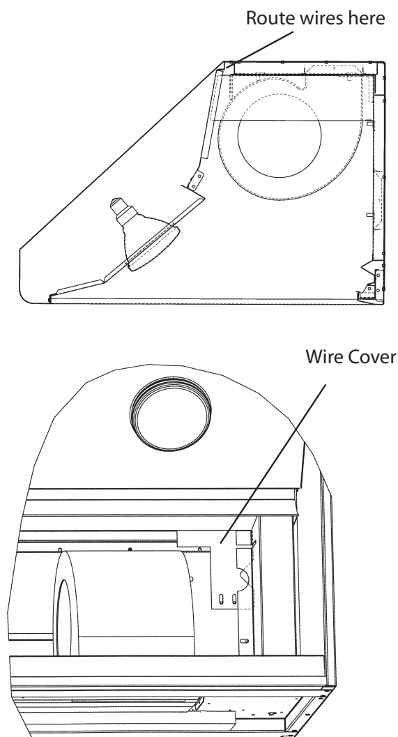
Figure 17: Vertical Discharge
