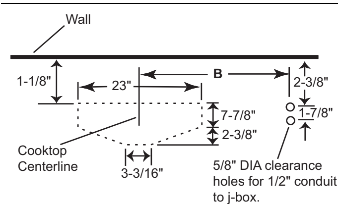
Plan View of Cabinet Cutout
