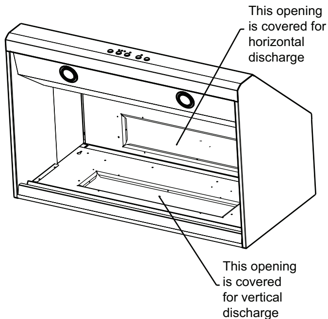
Figure 1: Discharge Direction
