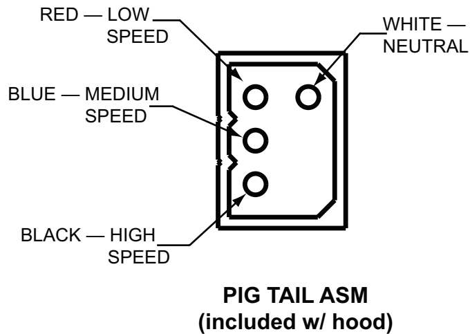
Figure 21: Wiring the Hood with an Inline Blower
