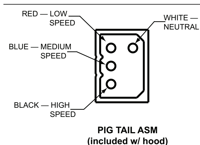
Figure 20: Wiring the Hood with a Remote Blower
