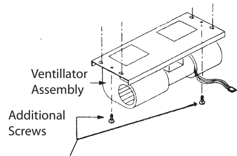
Figure 16: Attachment of Additional Screws
