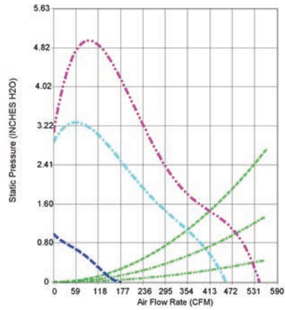
VTN600F-600 CFM
