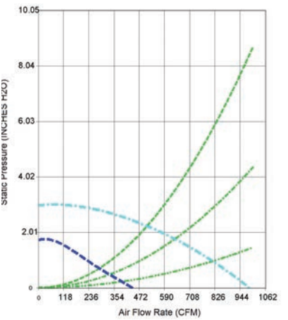
VTN1030N-1000 CFM
