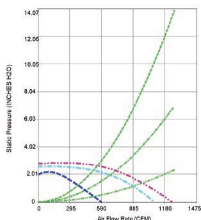
VTR1330E-1300 CFM
