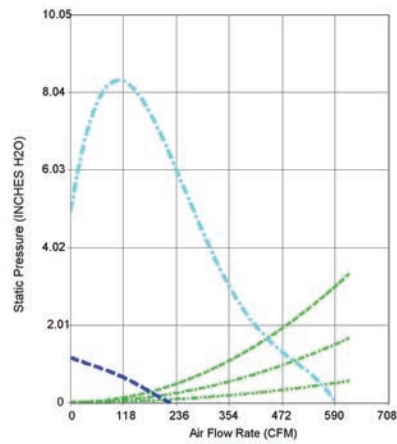
VTN600CV2C-600 CFM
