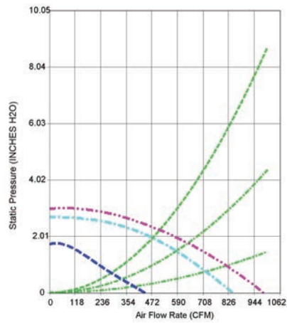
VTN1080N-1000 CFM
