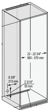
Cut out dedicated cabinet box
