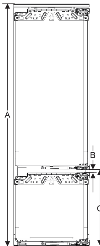
Fig. 66 Clearances for a 2-door cabinet door
