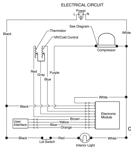
SYSTEM SCHEMATIC
