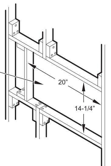
FRAME CONSTRUCTION
