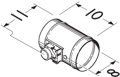
Model MD8T Model SMD8 Model MD8TR
