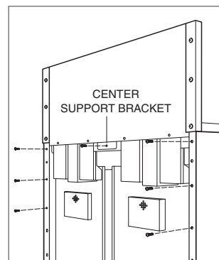
Insert riser supports.
