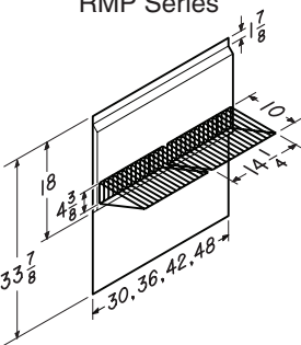
Backsplash RMP Series
