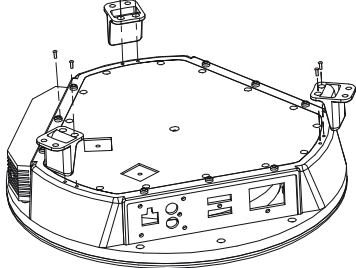
Attaching the mounting legs to the ends of the enclosure.
