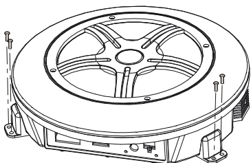
Attaching the mounting brackets to the mounting surface.
