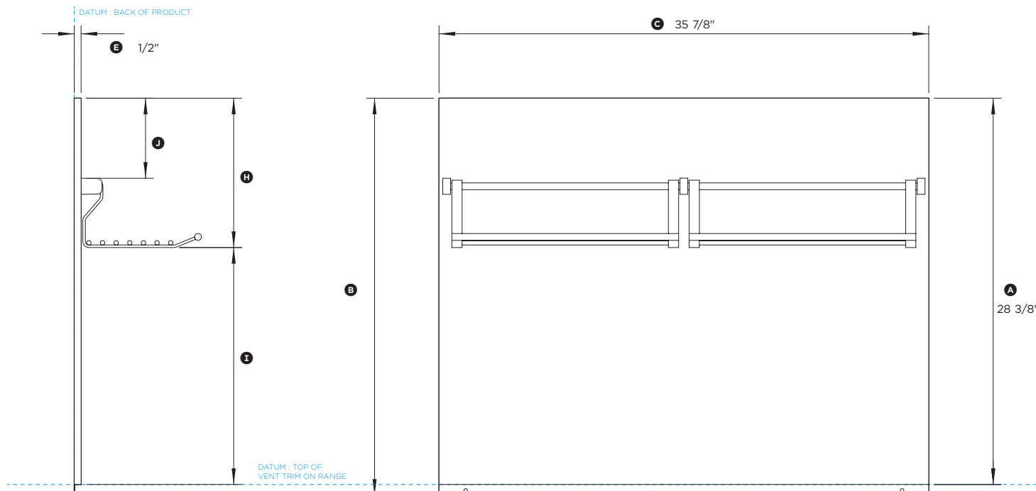
PROFILE VIEW
