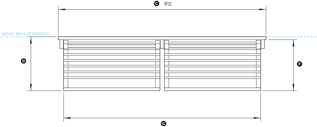
PLAN VIEW
