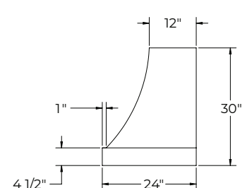
48" SIDE VIEW
