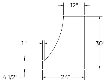
36" SIDE VIEW
