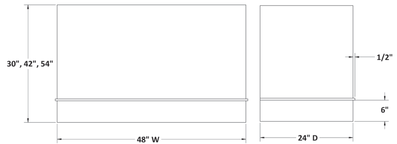
48" FRONT VIEW (49" WIDTH WITH 1/2" BANDS)
