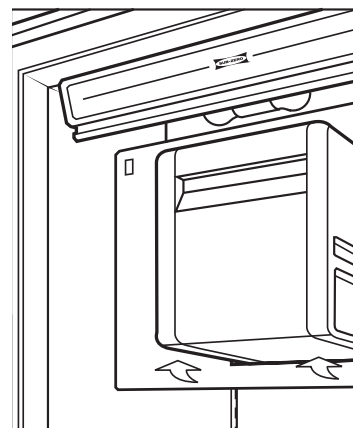
Ice bucket removal – Models 685 and 695
