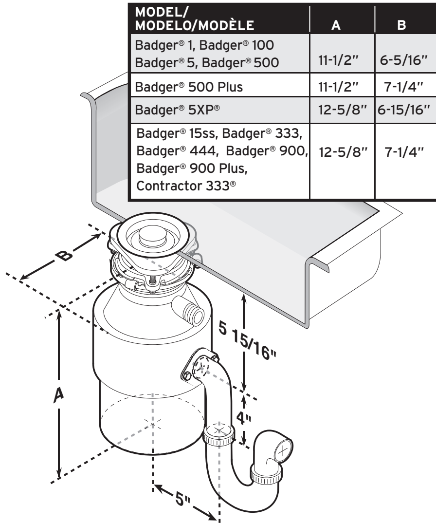
Dimensions/Dimensiones/Dimensions
