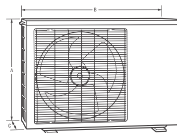
FFHP223CS2 1 Outdoor
