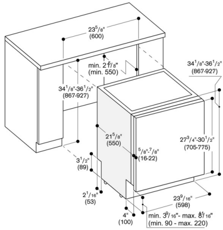
Tall Tub dishwasher (34" (86.7 cm)).
