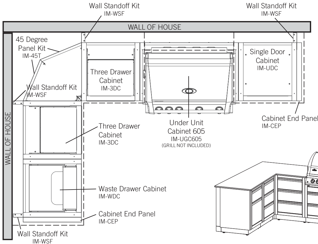
Oasis™ Modular Island Sample
