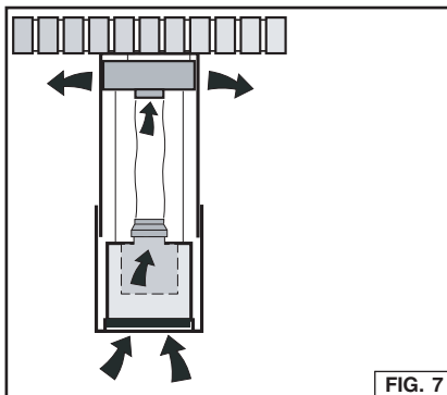
Non-Ducted with Decorative Flue Covers (requires AEIC35SB Ducted & Non-Ducted Flue Kit). Fig. 7.
