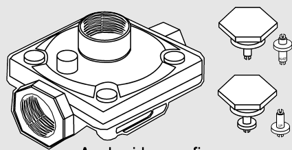
Apply sideways finger pressure to remove pin from cap.
