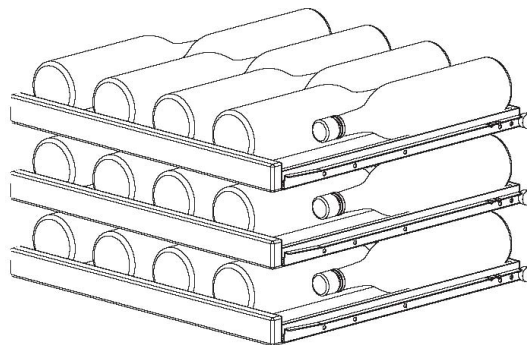
Figure 21 MPRO6WCM 8 bottles of wine per rack
