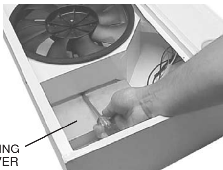
DAMPER/DUCT CONNECTOR
