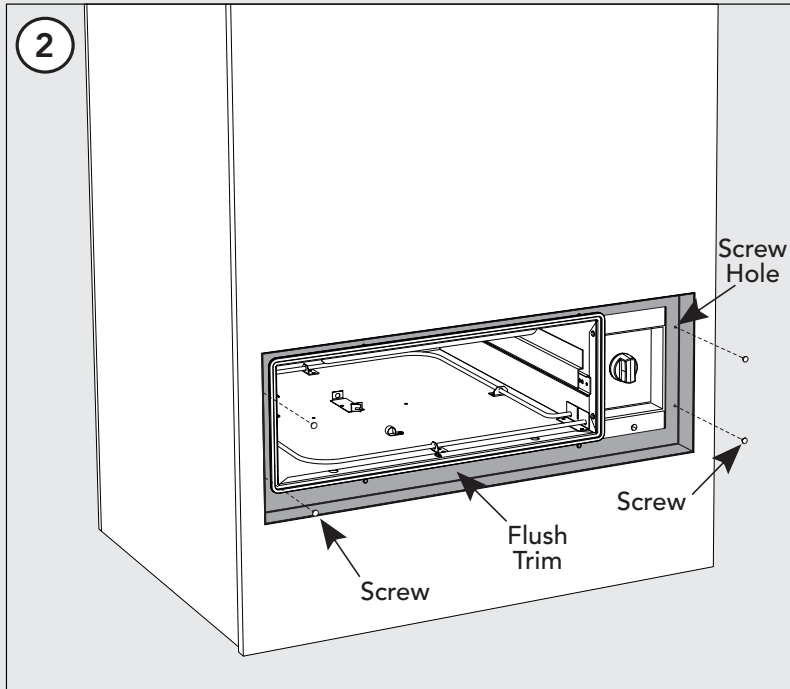
After installing the flush kit on the warming drawer, push the unit into the cutout. The flush kit will rest against the vertical blocking. Screw the flush trim to the vertical blocking with 4 screws as shown above.
