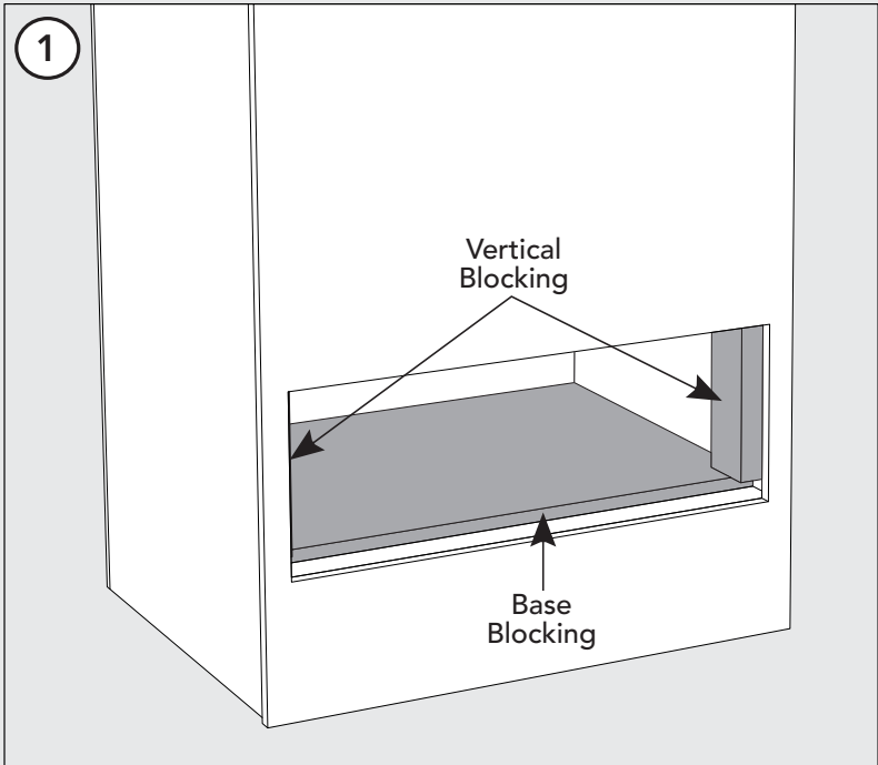
Install the vertical blocking and base blocking into the cutout area.
