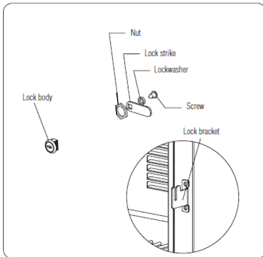
Figure 6. Door Lock
