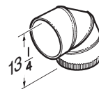
Model 418 10" Round 90° Elbow
