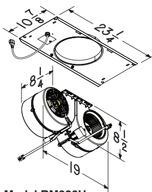
Model RM326H Blower / Rough-in Kit
