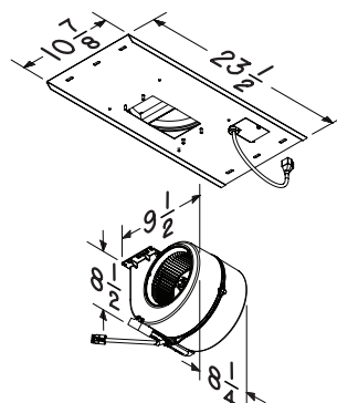
Model RM325H Blower / Rough-in Kit
