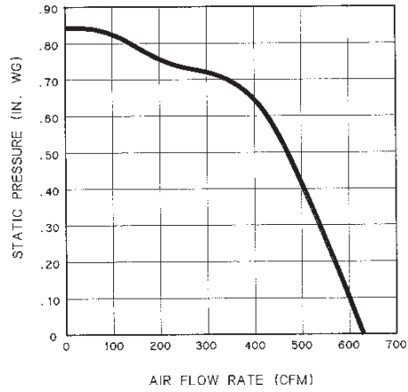
MODEL 331H EXTERIOR BLOWER
