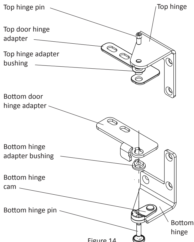
Figure 14 Right hand hinges shown
