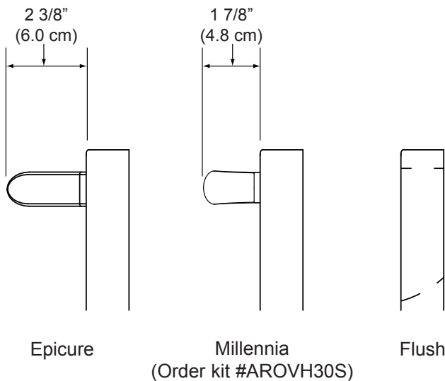
Handle Dimensions
