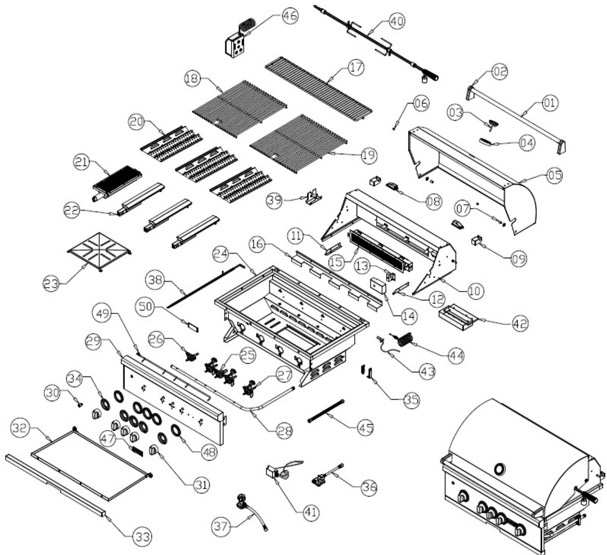
CSX36 and CSLX36 Parts Listing
