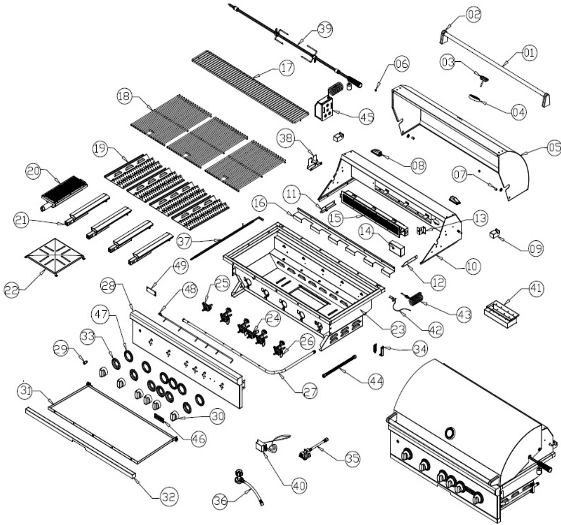
CSLX42 Parts Listing
