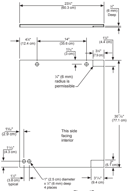
Figure 17 Left Hand Hinged Door 24" (61 cm) wide appliance
