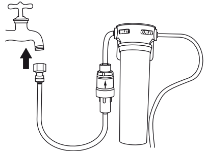
Diagram 3 Faucet connection
