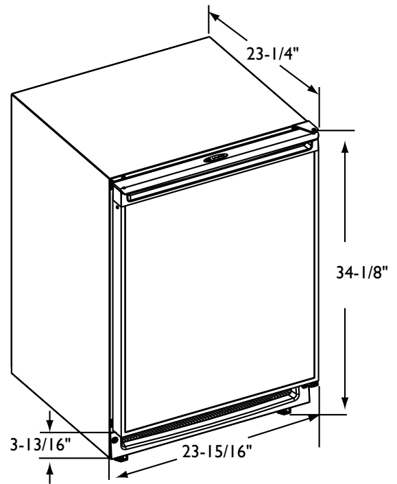
2175RCB Black Model and 2115RCW White Model
