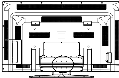
Screws: 6xM4x12
