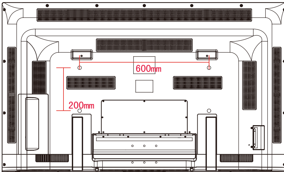
Dimensions for Mounting Hole Pattern
