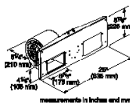
VTN630C—600 CFM
