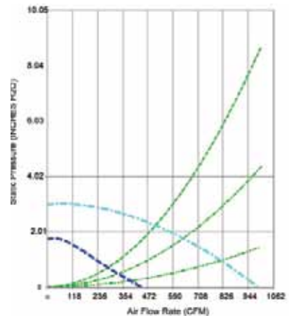
VTN1030C – 1000 CFM
