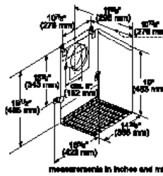
VTR630D—600 CFM
