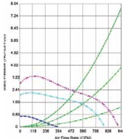
VTN1000F – 1000 CFM
