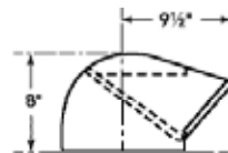
Roofjack–RJ310
