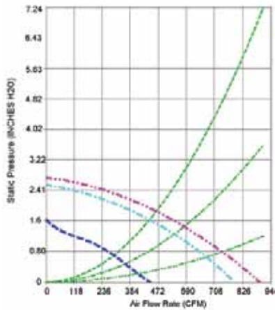
VTR1030D-1000 CFM
