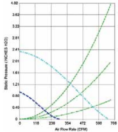
VTN630C – 600 CFM
