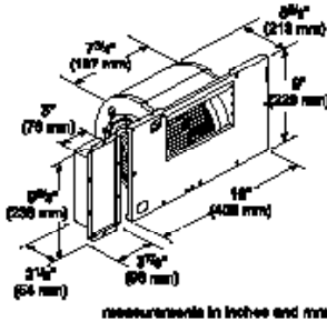
VTN1000F – 1000 CFM
