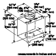
VTI610D—600 CFM
