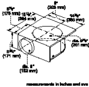
VTN1080F – 1000 CFM
