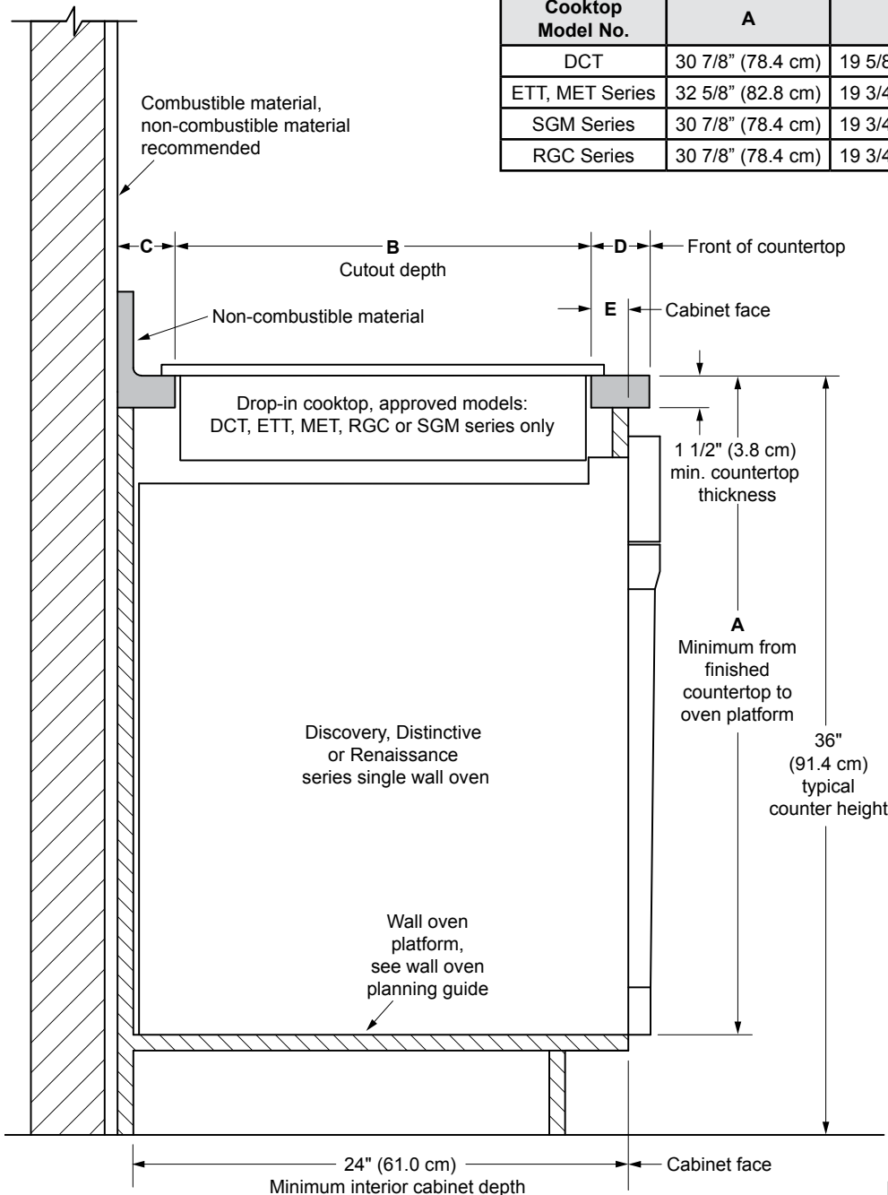
CUTAWAY SIDE VIEW
