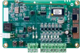
RAK364R1—Chassis-Mounted Receiver (AZ2500, 2800, 2900, 4100, 7500 and 8500 series*) Electric Heat Wireless Remote Receiver
