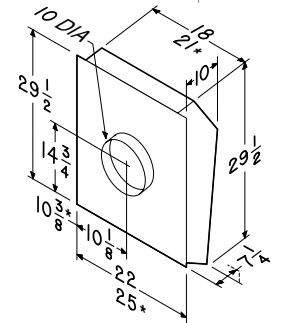
Models 335 & 336 Exterior Blowers
