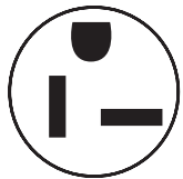
*Plug Type (NEMA) (C) 6-20P
